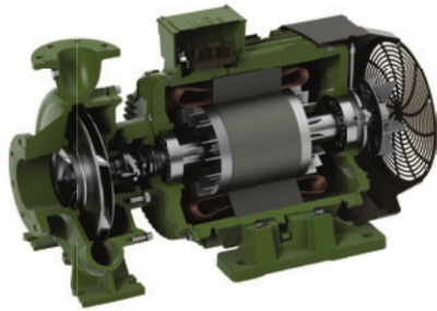
NCB - NCBK LONG - COUPLED VERSION
